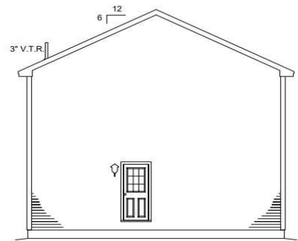
LEFT ELEVATION
