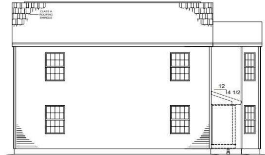
LEFT ELEVATION
